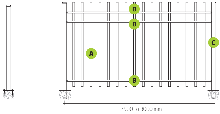
Pate Metal Concrete Foundation
